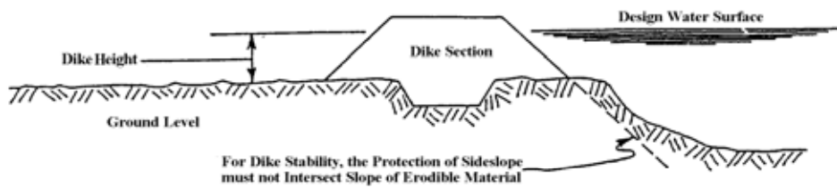
FIGURE 12. Dike Cross-Section
