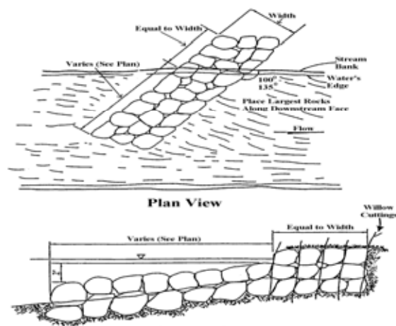
BARB DETAILS No Scale
